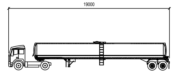
FH 13 4x2 Low WB 3600 - Walker Foodliner
